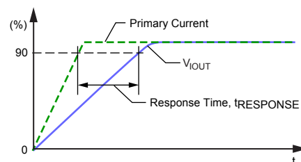
Figure 5: Response Time ( t_{RESPONSE} )
